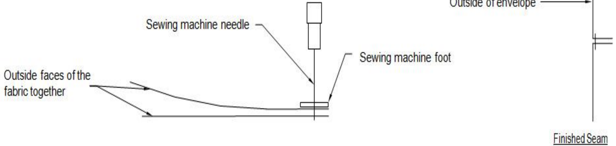
Fig. 3 Seam Detail
