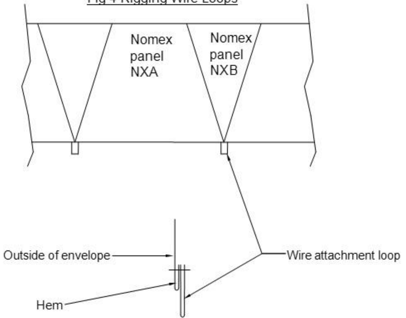
Fig 4 Rigging Wire Loops
