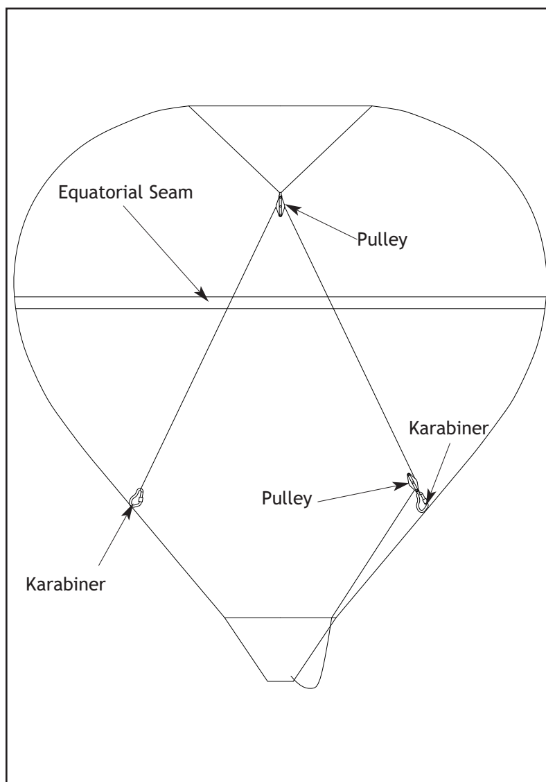
▲ Fig 2: Connect System General Arrangement
